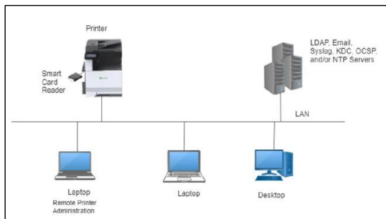
Figure 1: TOE Architecture
